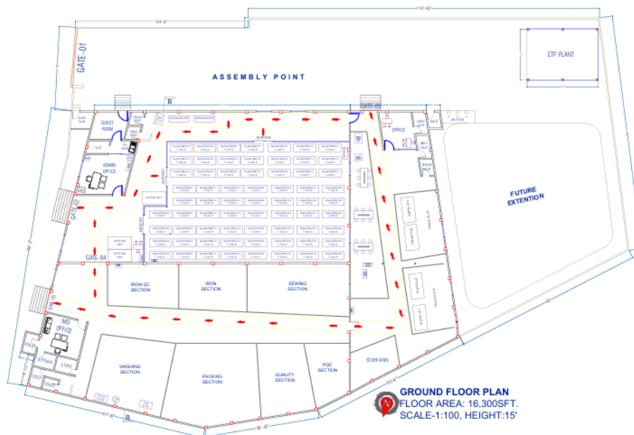
Ground Floor Plan — Floor area 16,300 sq. ft. · Scale 1:100 · Height 15'
